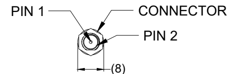
VIEW B 2 PIN FEMALE MATING FACE
