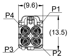
VIEW A 4 PIN FEMALE MATING FACE
